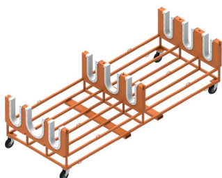
WSPA-186 Transport mount for removed elevators and rudders
