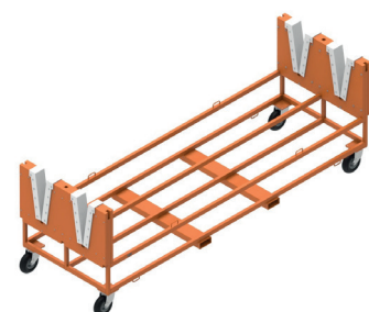
WSPA-191 Dolly for aileron transport
