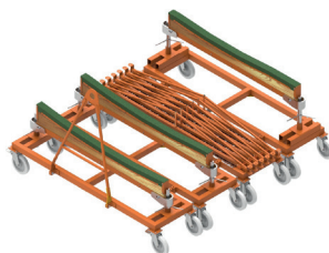
WSPA-184 External wing dolly (folded for storage in a hangar)
