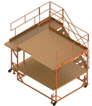
UW-4-BF Rear right platform for aircraft maintenance
